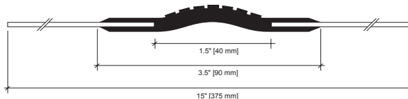
DILA GS -Galvanized Steel - Exposed Gland
