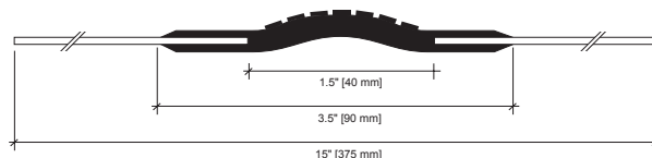
DILA-Pb (Lead) - Exposed Gland
